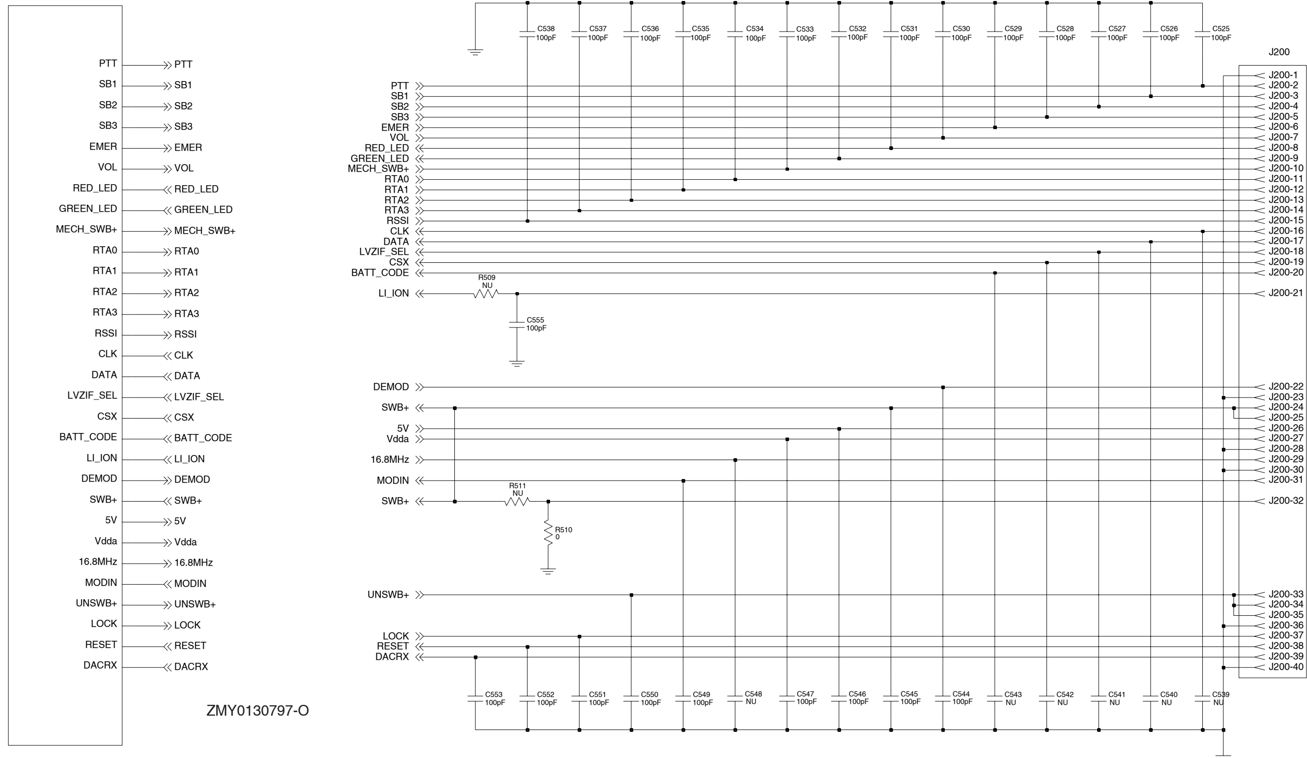
UHF Band 2 Controls And Switches Schematic Diagram (sheet 1 of 2)
